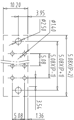
PCB Layout
